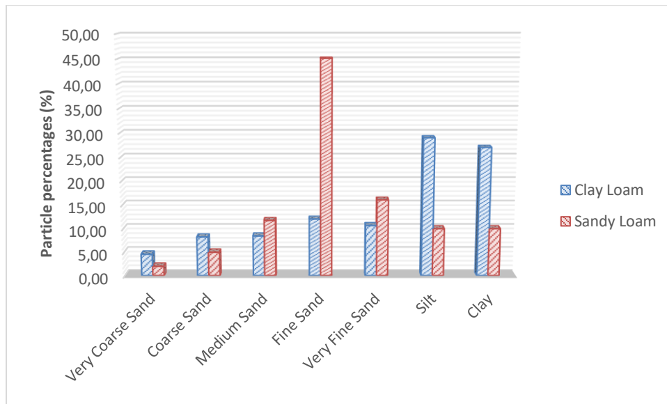
Figure 1.P article size distribution of the soils
